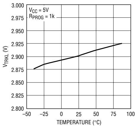
Trickle Charge Threshold vs Temperature
