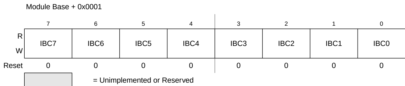
Figure 10-4. IIC Bus Frequency Divider Register (IBFD)
