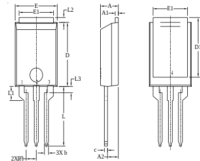
PLUS220 (IXFV) Outline
