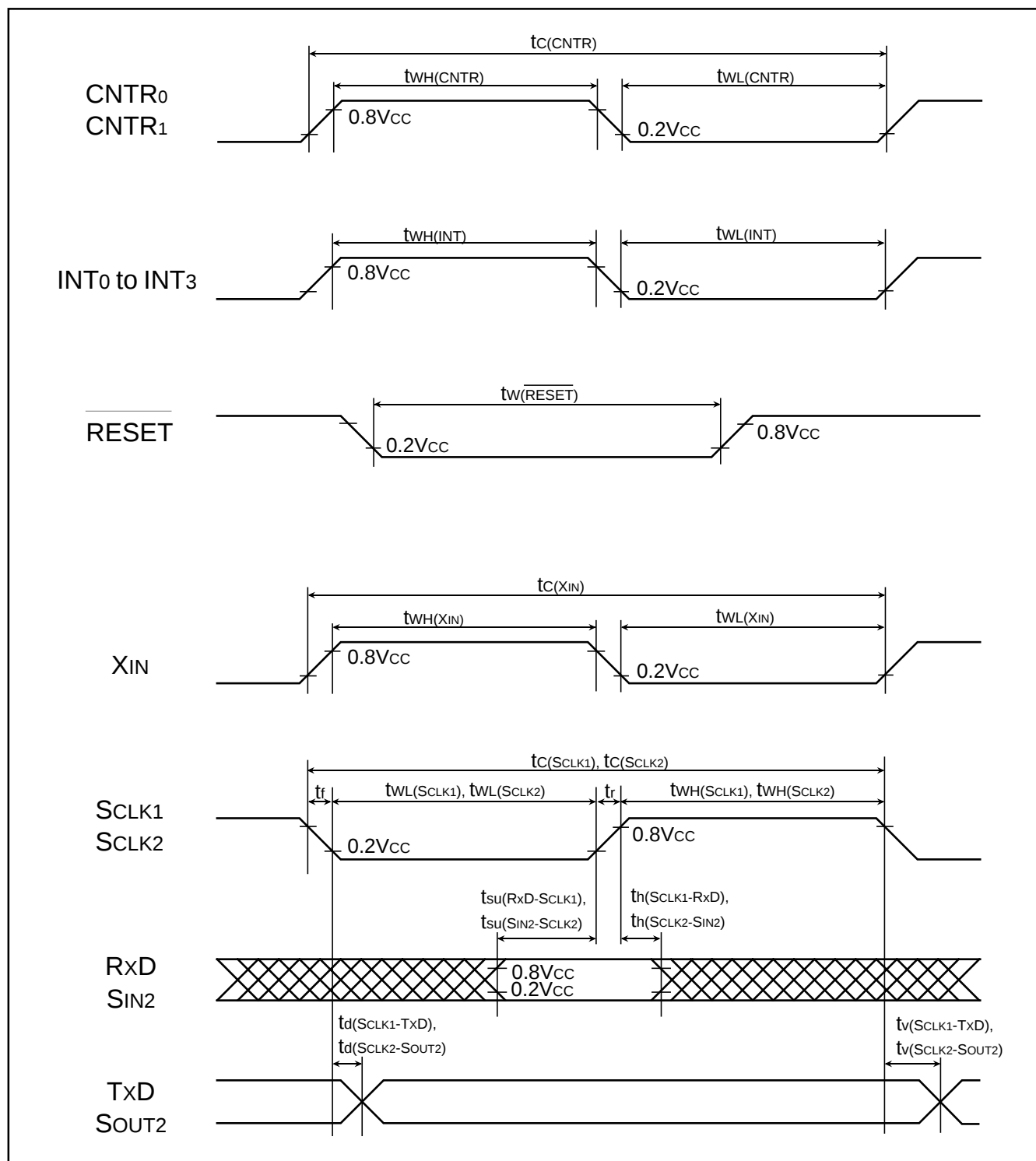
Fig. 60 Timing diagram
