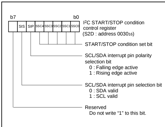
Fig. 38 Structure of I²C START/STOP condition control register
