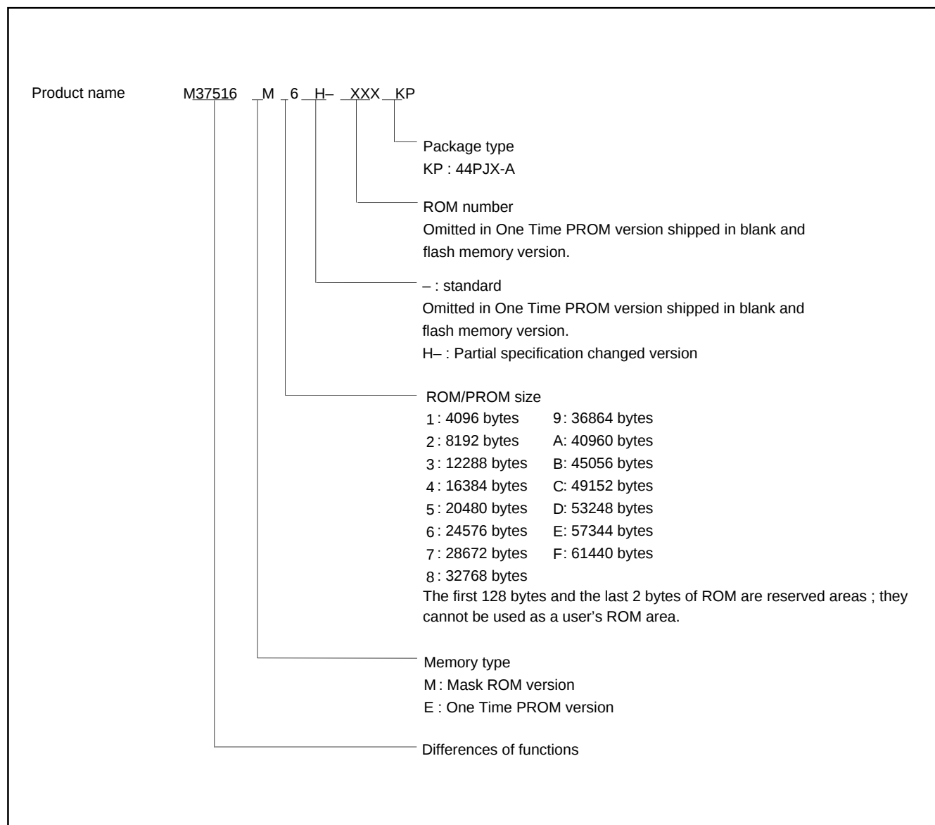
Fig. 3 Part numbering
