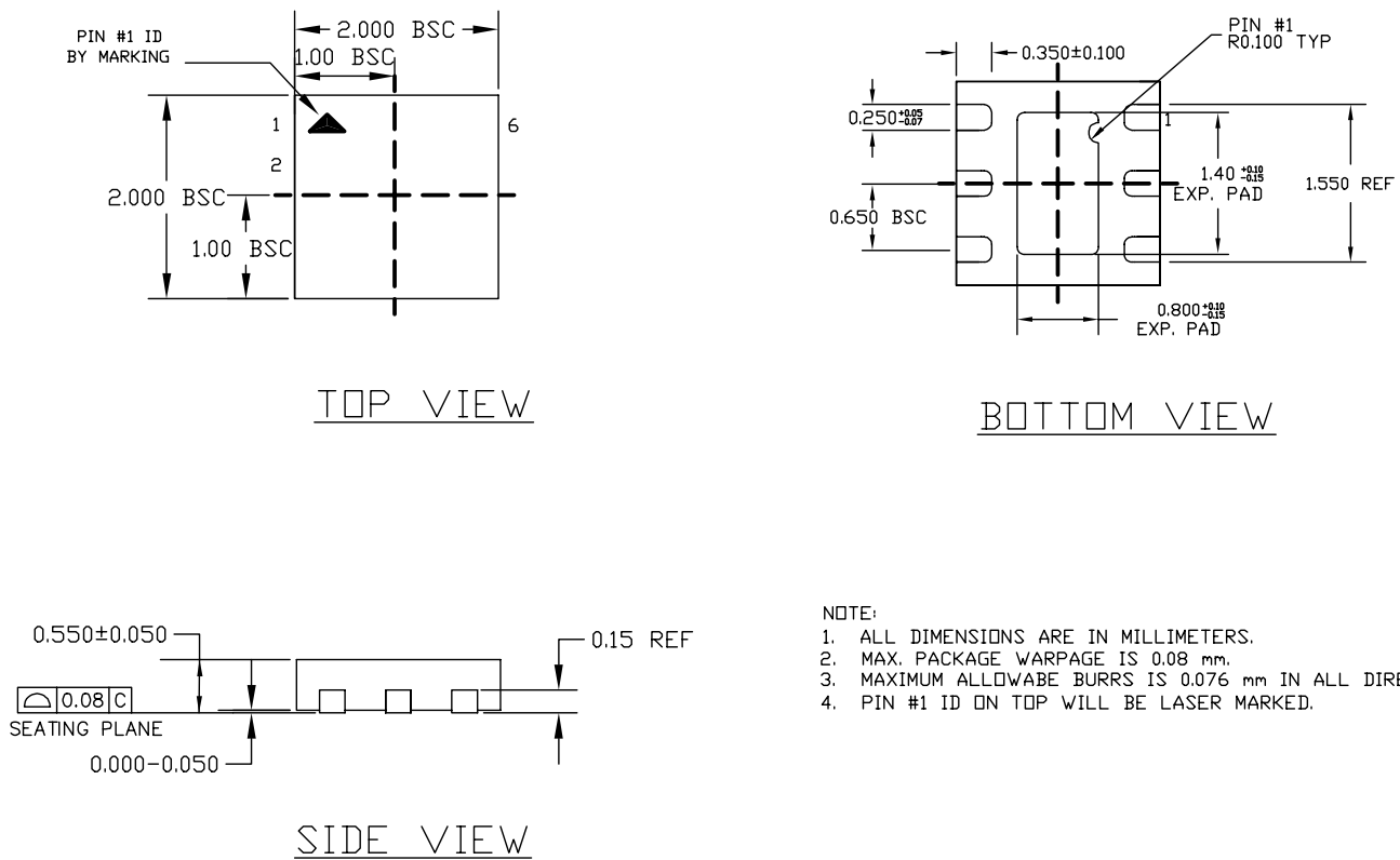
6-Pin 2x2 Thin MLF ® (MT)
