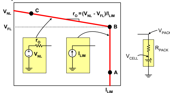
FIGURE 26. THE IDEAL I-V CHARACTERISTICS OF A CURRENT LIMITED ADAPTER
