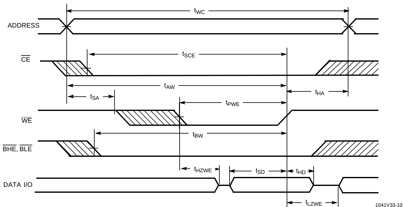
Write Cycle No.3 ( \overline{\text{WE}} Controlled, \overline{\text{OE}} )
