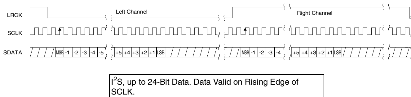
Figure 18. CS53L32A Control Port Mode - Serial Audio Format 0 (I 2 S)
