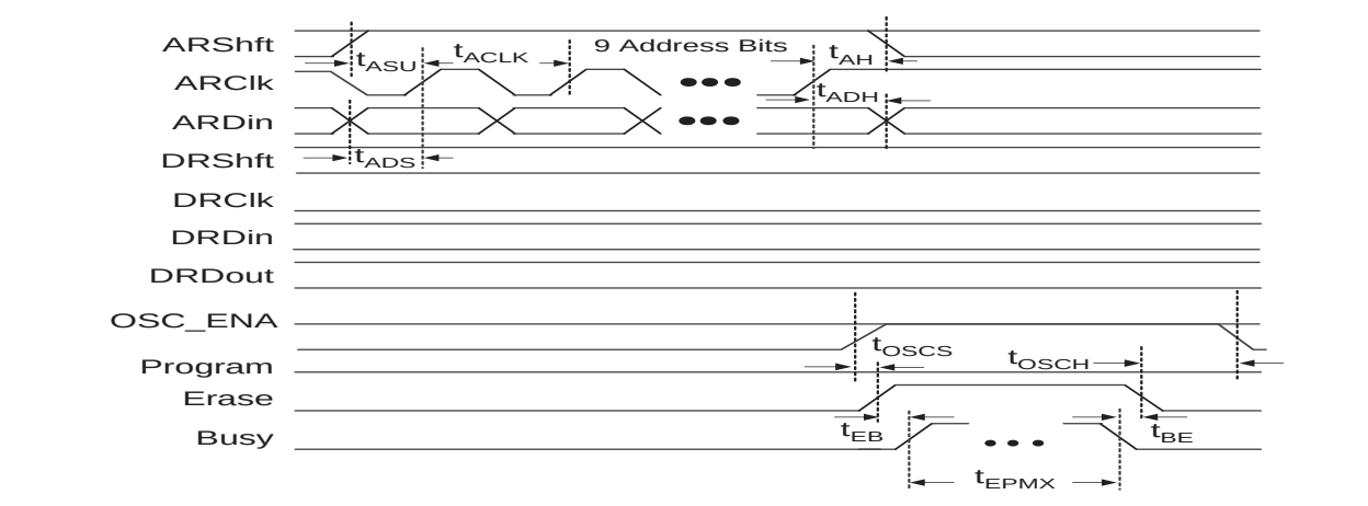
Figure 5-5. UFM Erase Waveform
