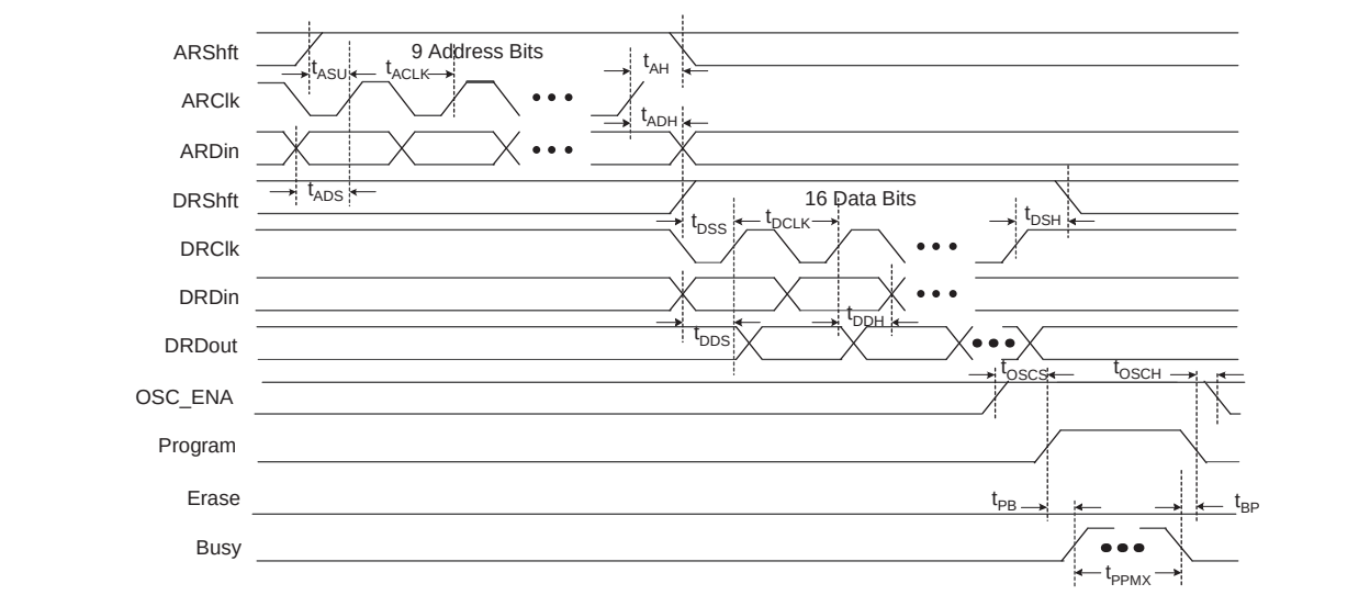
Figure 5-4. UFM Program Waveforms
