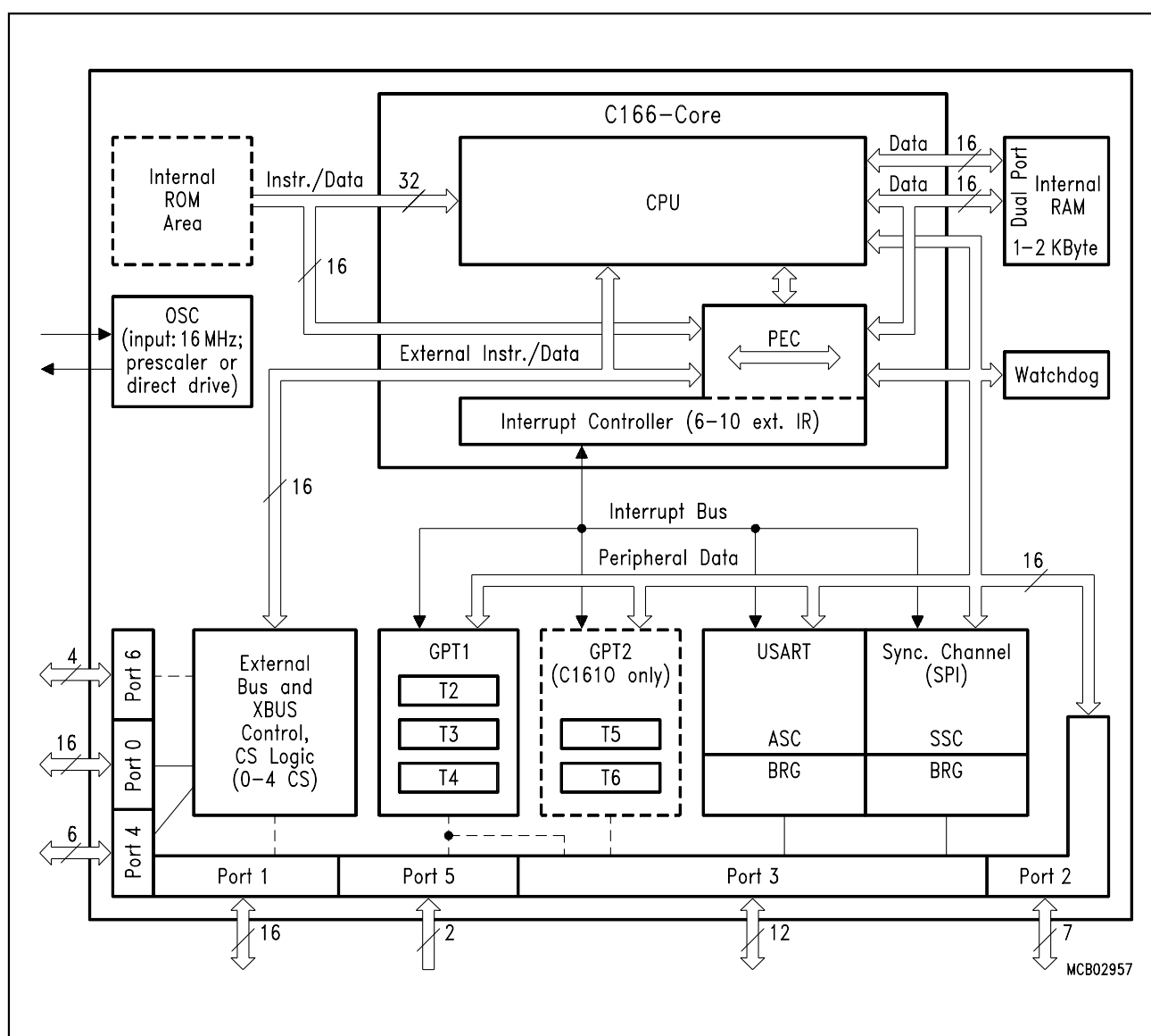
Figure 3 Block Diagram
