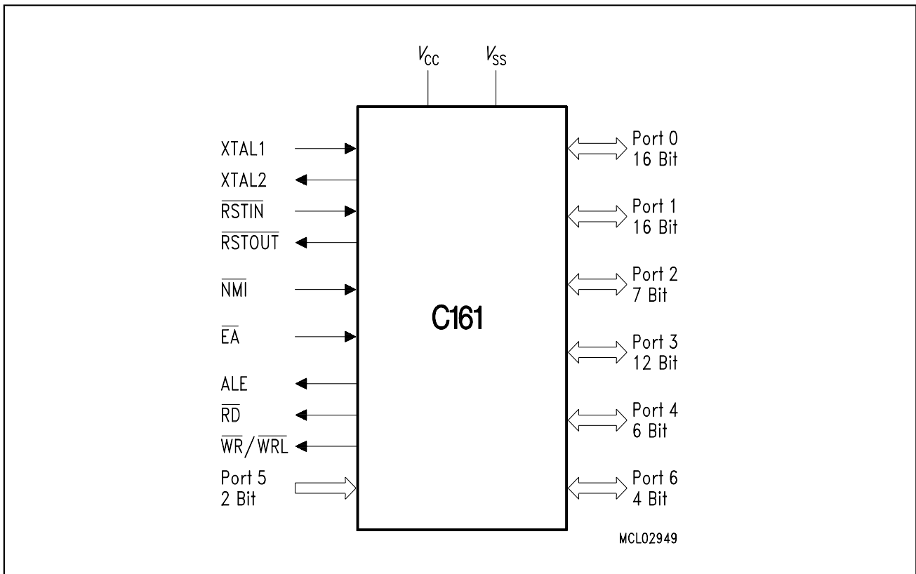
Figure 1 Logic Symbol
