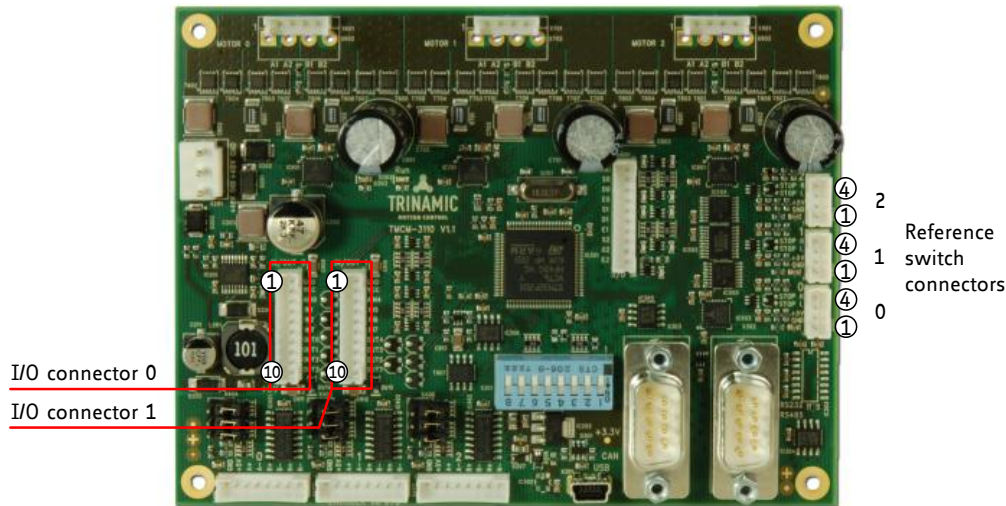
Figure 4.3 TMCM-3110 connectors
