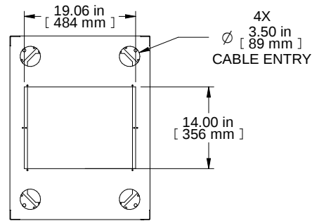
TOP VIEW TOP OPENING
