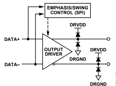
Figure 67. Digital Outputs
