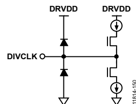
Figure 66. Equivalent DIVCLK Output Circuit (DRVDD)
