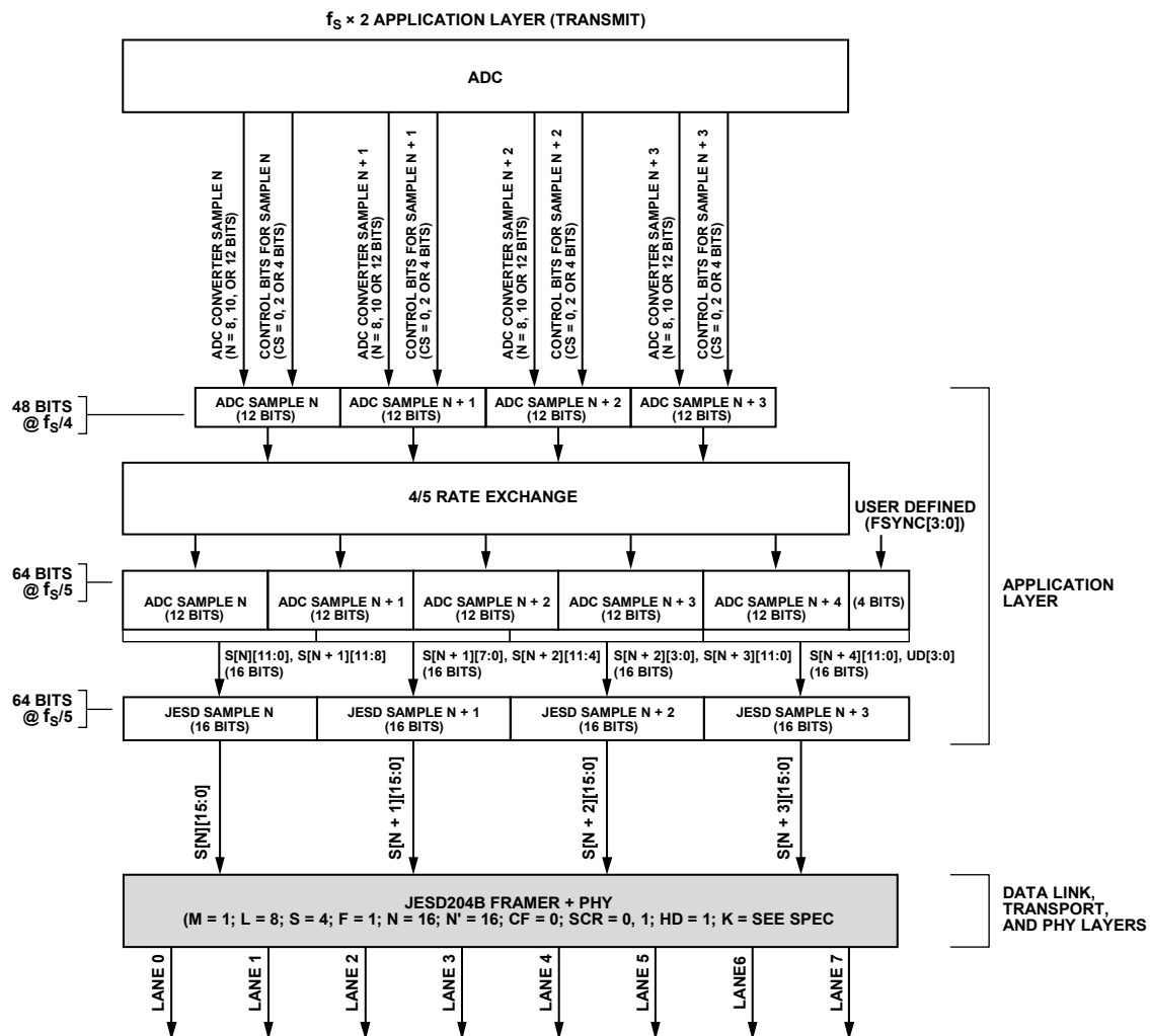
Figure 104. f_s \times 2 Mode Application Layer (Transmit)
