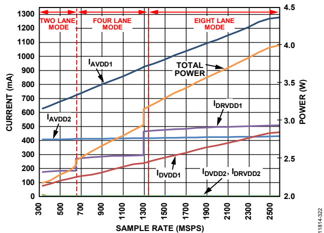
Figure 7. Current and Power vs. Sample Rate: Two Lane, Four Lane, and Eight Lane Output Modes
