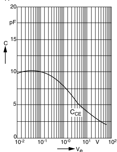
Figure 2. Transistor Capacitance (typical) vs. Collector-emitter Voltage T_A=25^\circ\text{C} , f=1.0\text{ MHz}
