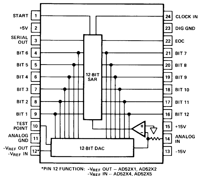
Figure 2. Pin Designations
