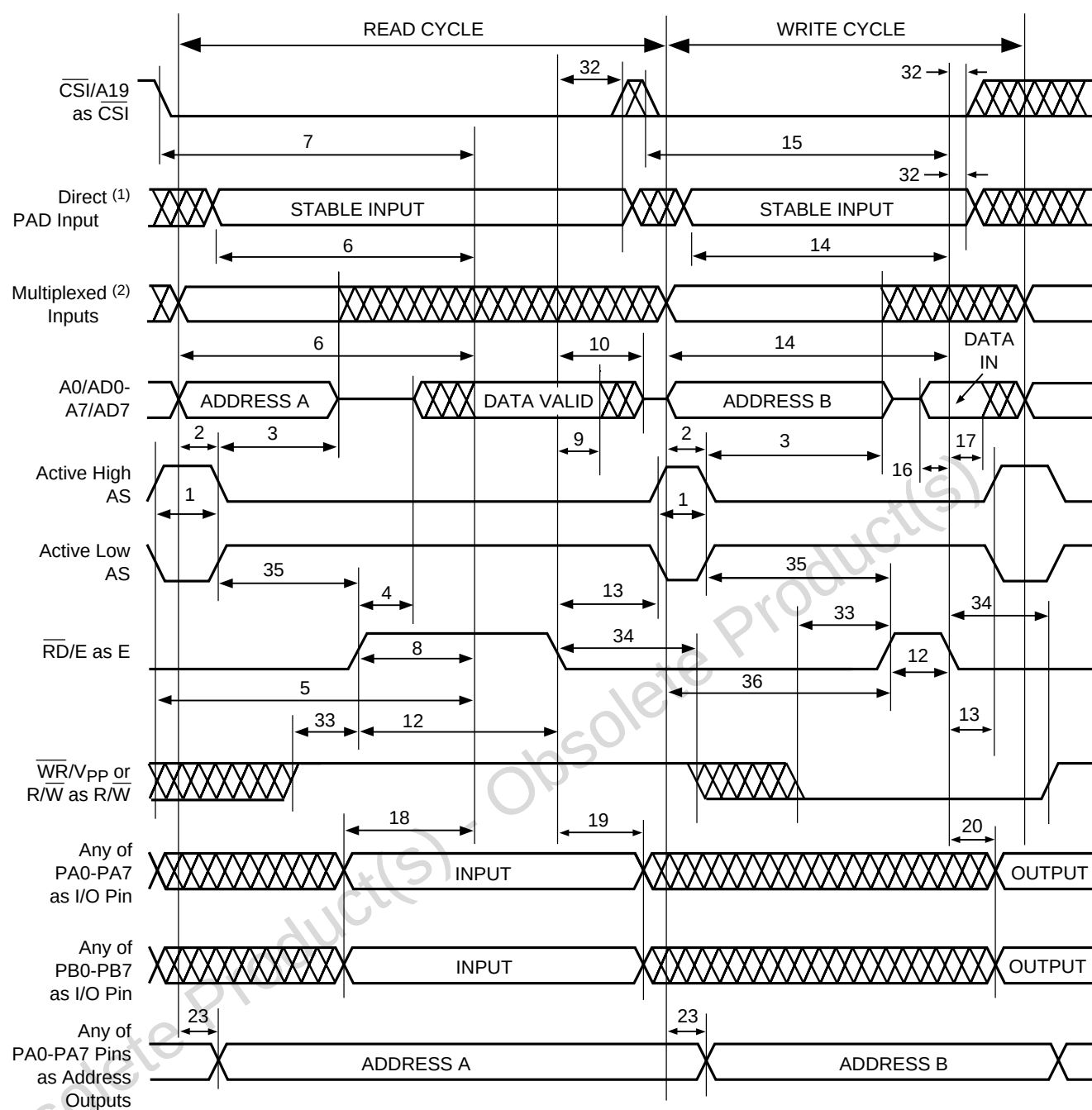
Figure 20. Timing Using \overline{R}/\overline{W} and E signals
