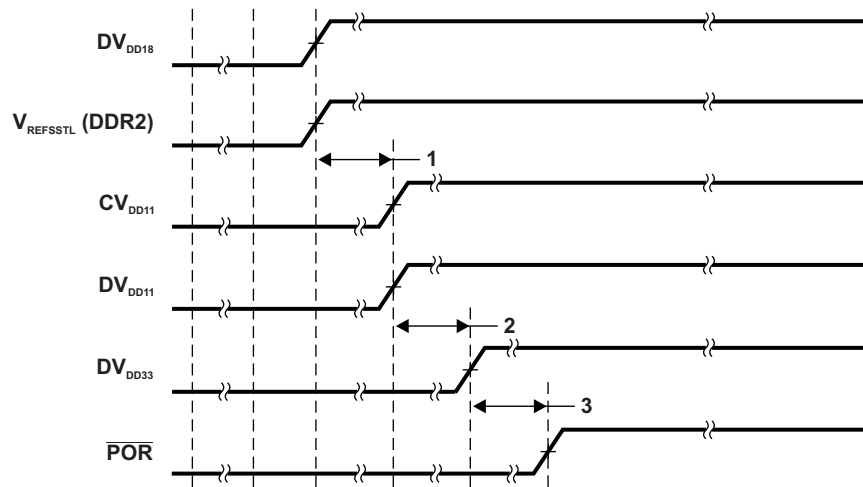
Figure 7-7 Power-Supply Sequence
