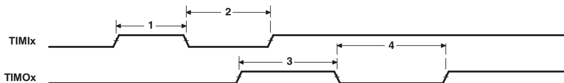
Figure 7-45 Timer Timing
