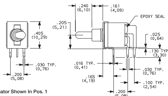
ET21MD1ABE Horizontal Actuation DPDT
