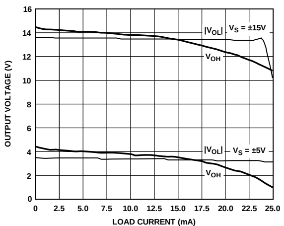
Figure 23. Output Voltage vs. Load Current
