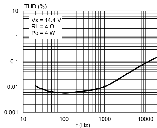
Figure 10. Distortion vs. frequency (4 \Omega )
