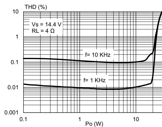
Figure 8. Distortion vs. output power (4 \Omega )
