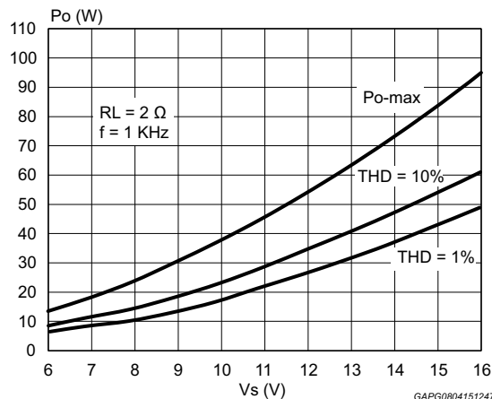
Figure 7. Output power vs. supply voltage (2 \Omega )
