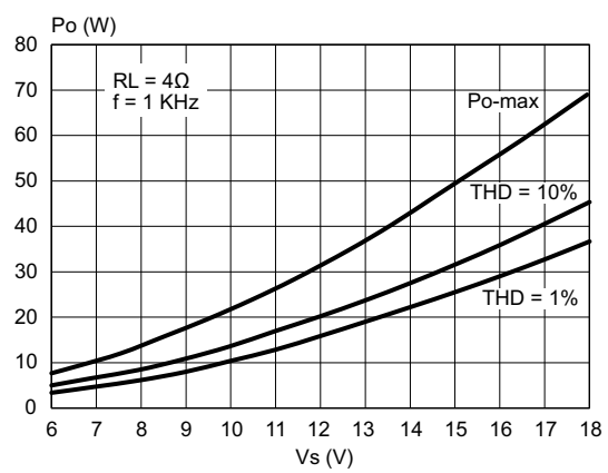
Figure 6. Output power vs. supply voltage (4 \Omega )
