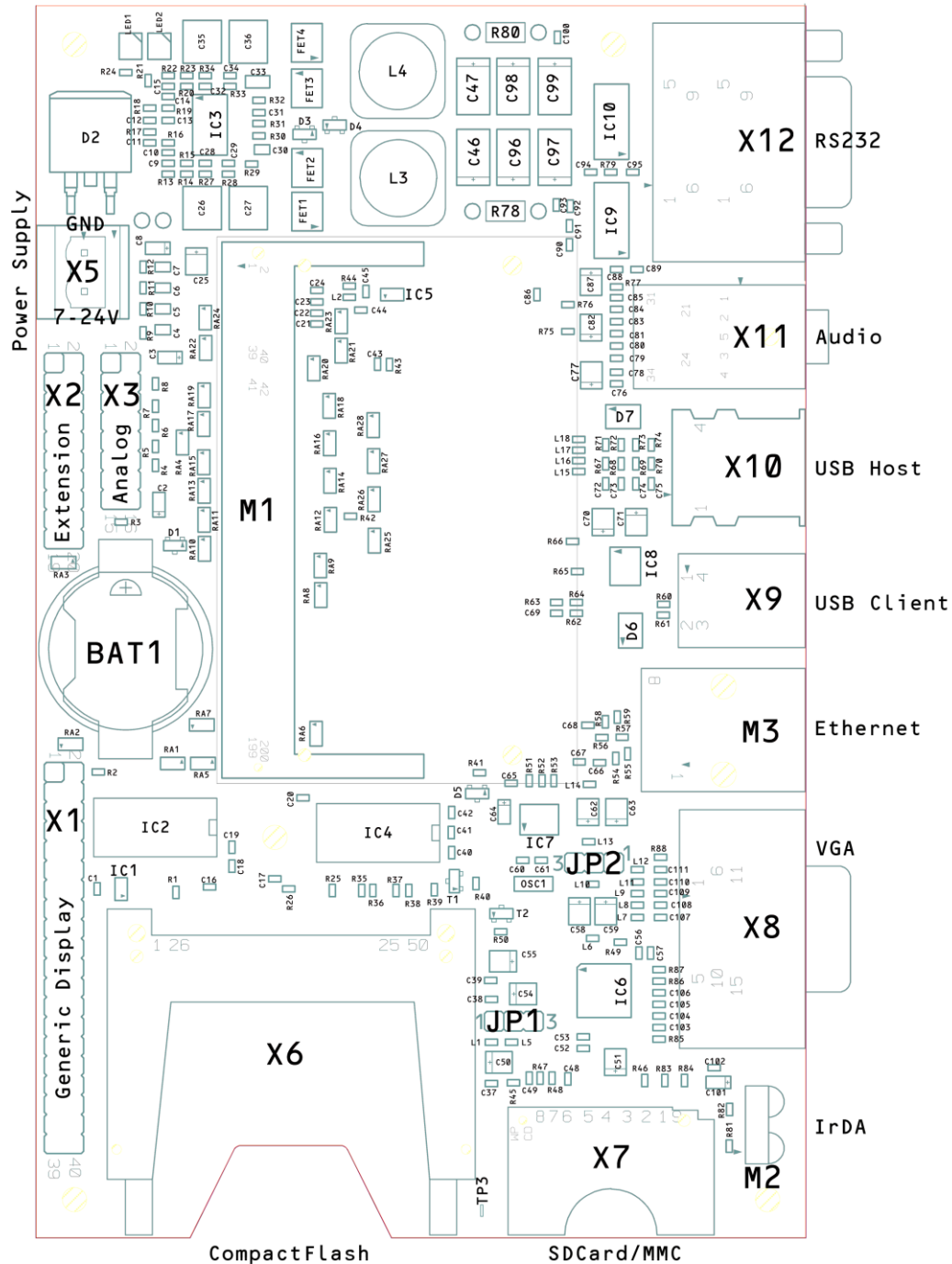
Figure 2: Orchid Layout: Top View
