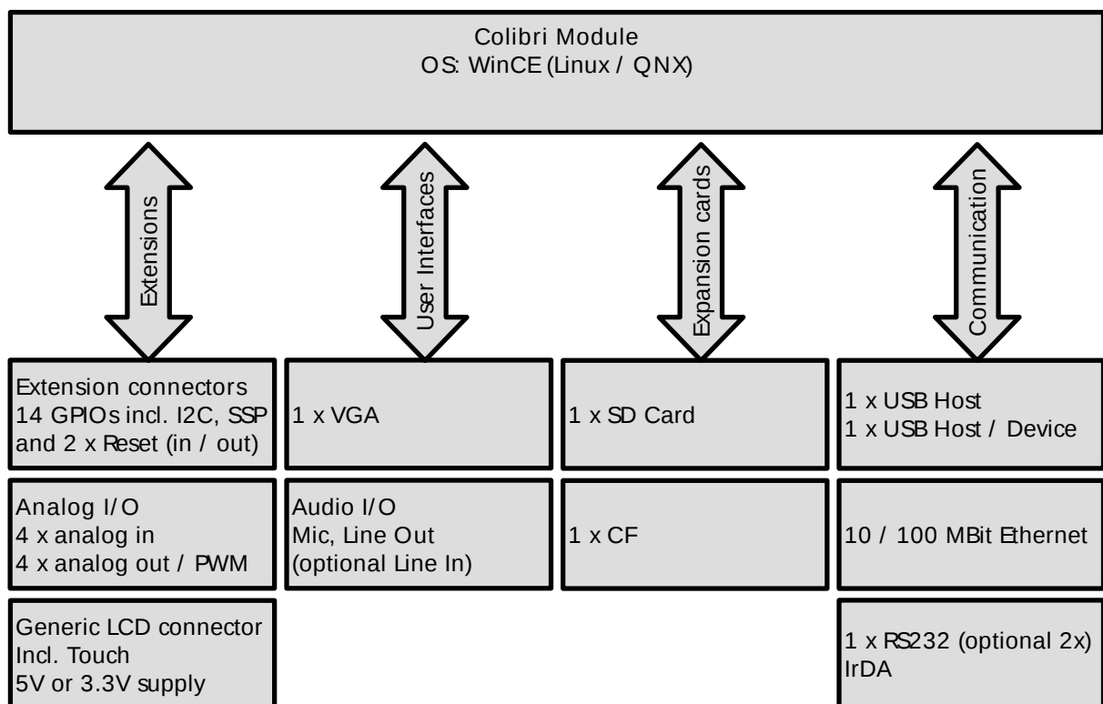
Figure 1: Orchid Block Diagram
