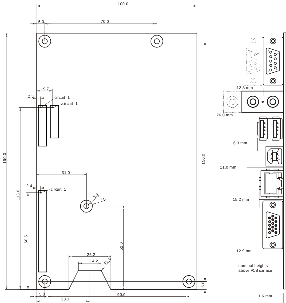
Fig. 3: Mechanical Drawing and Mounting Hole Positions
