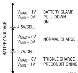
Figure 4. BAT Voltage Operating Range
