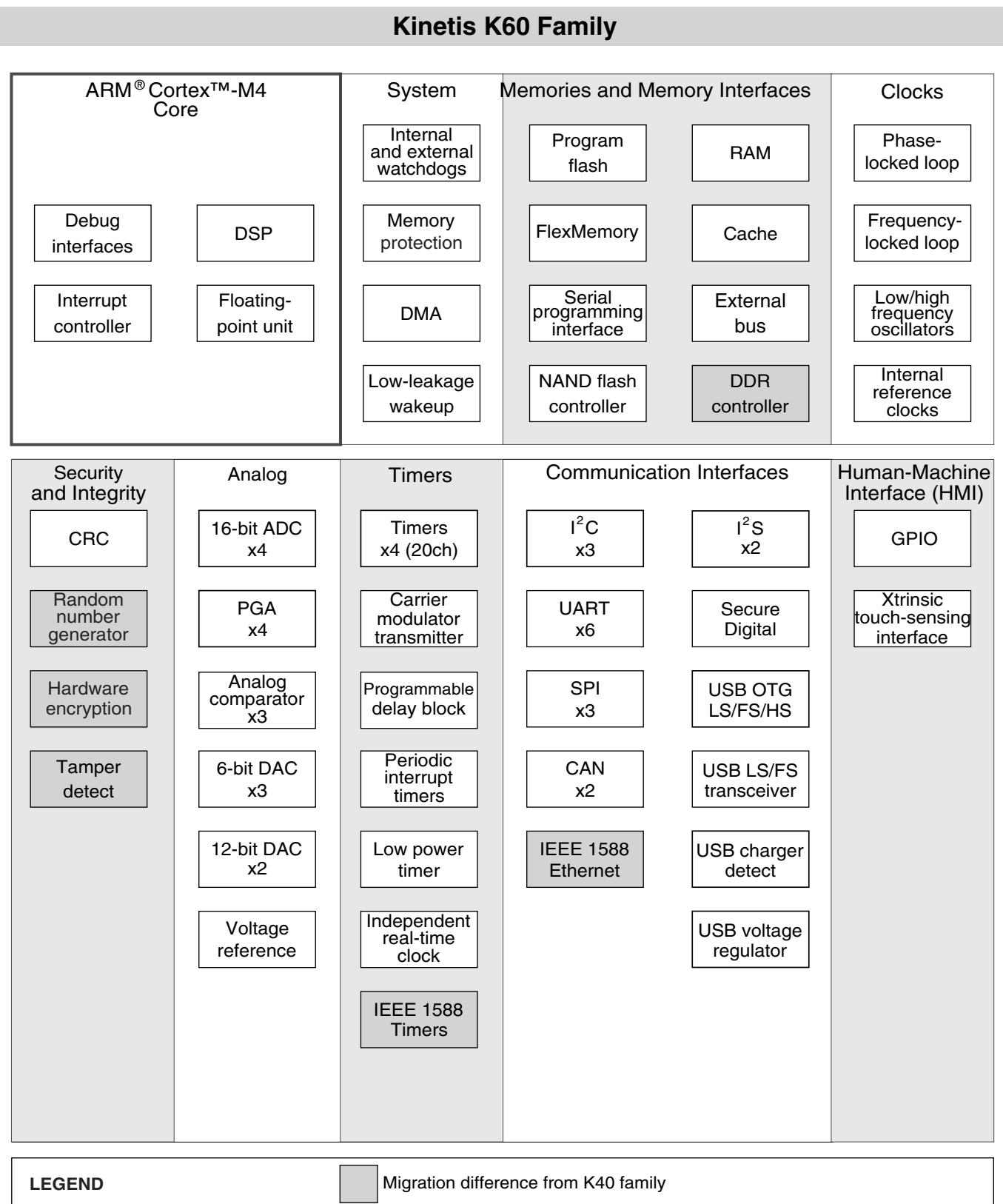
Figure 2. K60 Block Diagram
