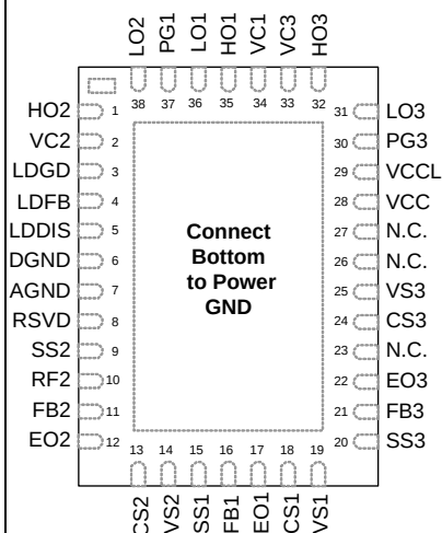
LQ PACKAGE (Top View)
