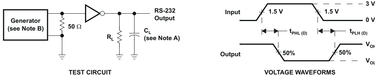
Figure 6-1. Driver Slew Rate
