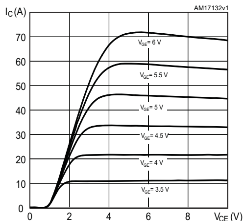
Figure 8. Output characteristics ( T_J = -40^\circ\text{C} )
