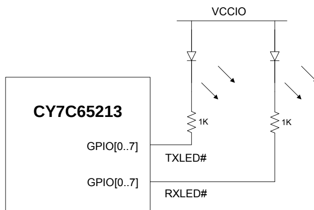
Figure 10. Double-LED Configuration
