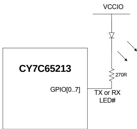
Figure 9. Single-LED Configuration
