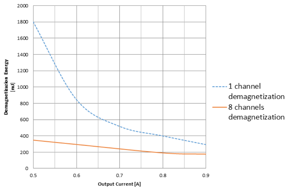
Figure 25. Single pulse demagnetization energy vs. load current (Typical values at T_{AMB} = 125^{\circ}\text{C} )
