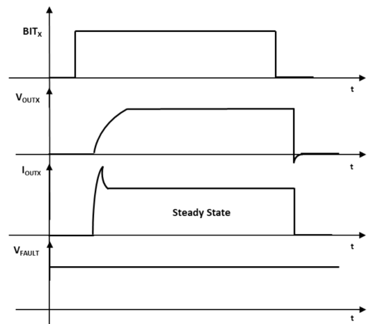
Figure 15. Switching on bulb lamp
