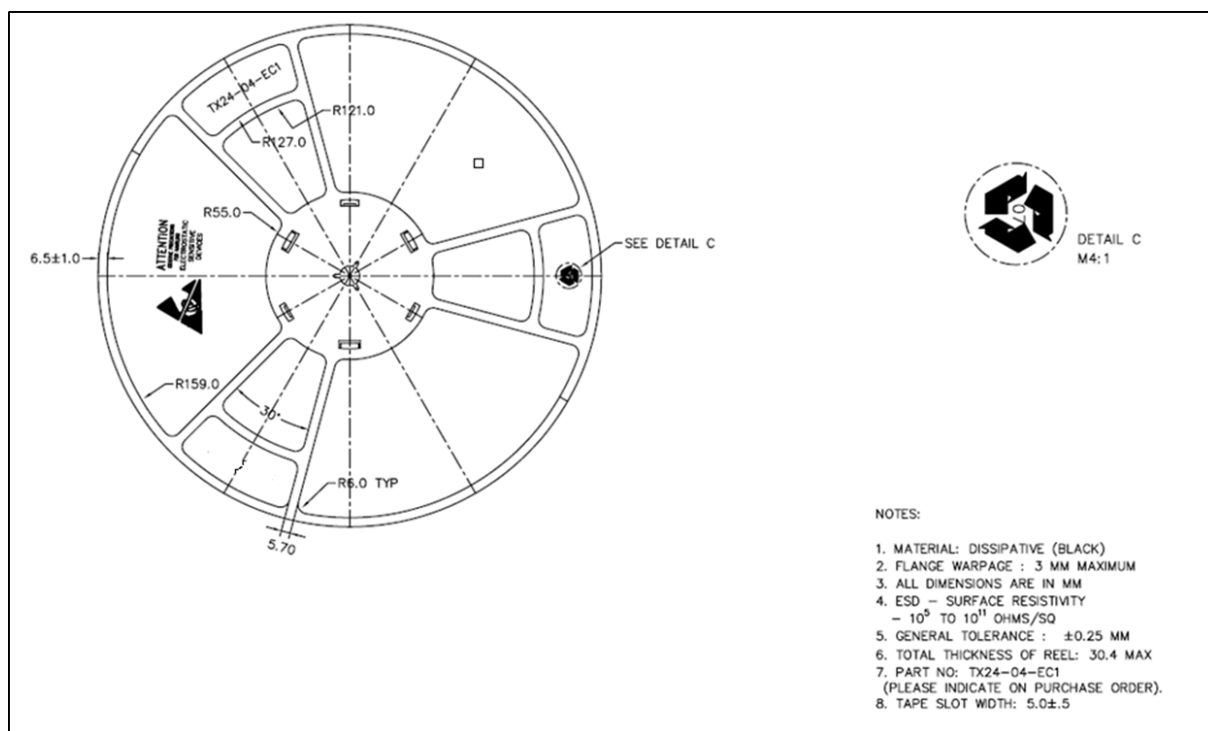
Figure 34. TFQFPN32 reel
