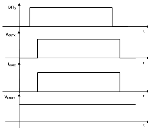
Figure 14. Switching on resistive load
