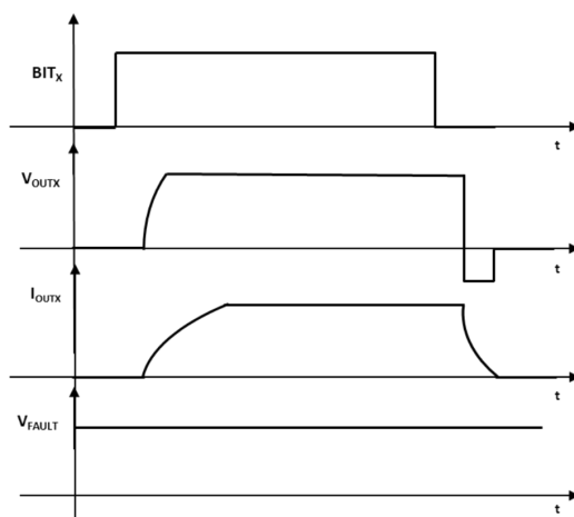
Figure 16. Switching on light inductive load
