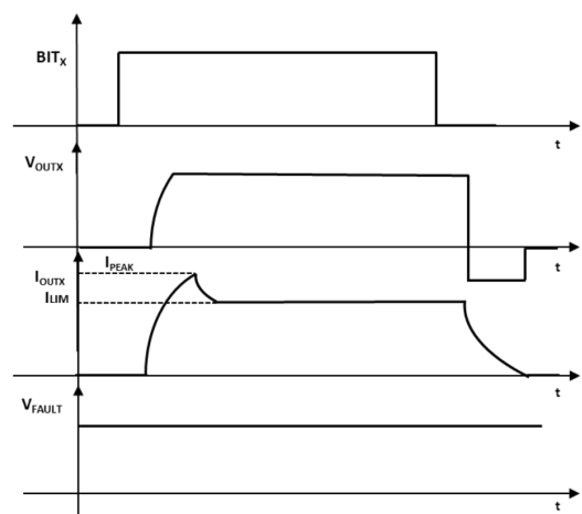
Figure 17. Switching on heavy inductive load
