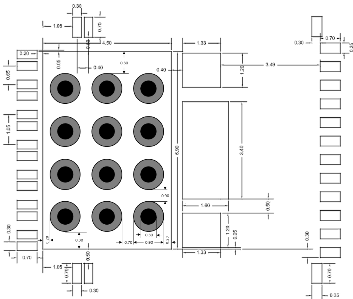
Figure 31. TFQFPN32 suggested footprint (measured in mm)
