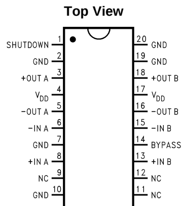
Figure 1. TSSOP Package See Package Number PW0020A
