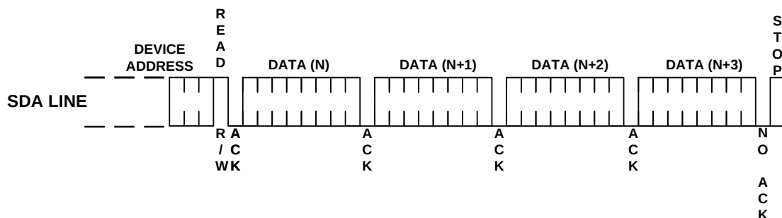
Figure 8: Sequential Read
