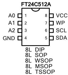
Figure 1: Package Type
