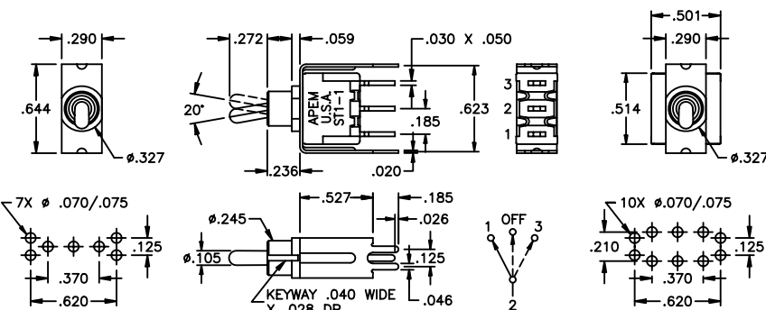
SINGLE POLE
