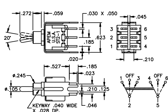
DOUBLE POLE
