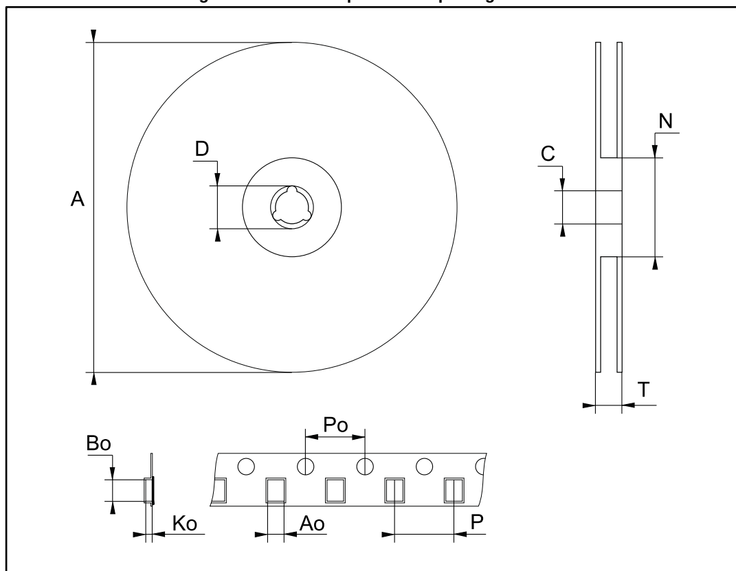
Figure 4: SSOP 28 tape and reel package outline
