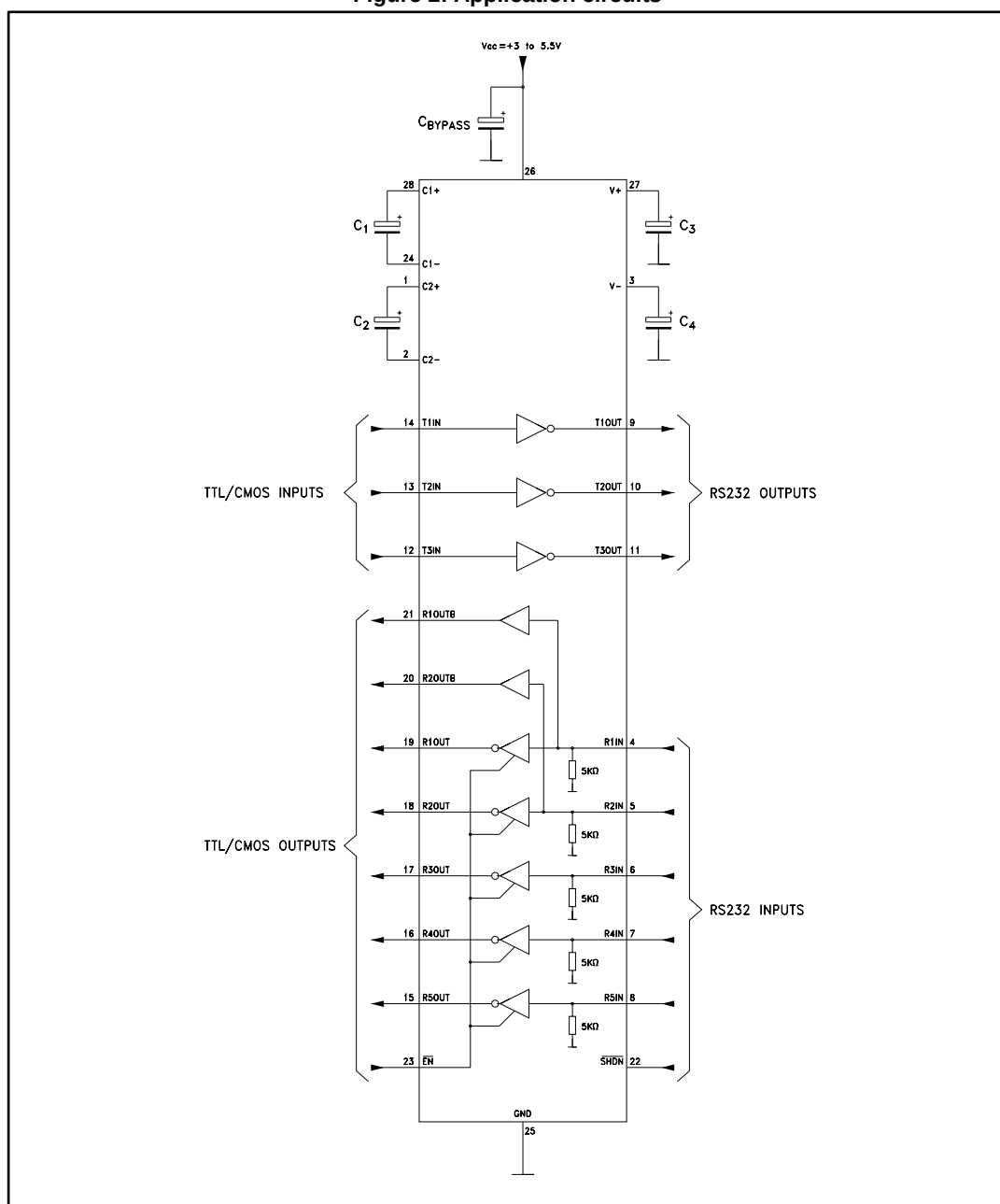
Figure 2: Application circuits
