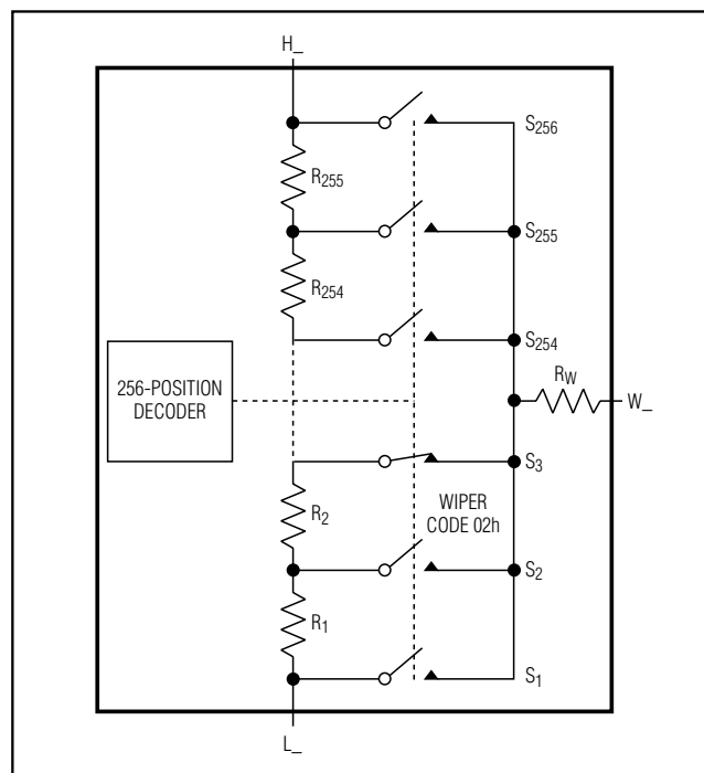
Figure 2. Potentiometer Configuration
