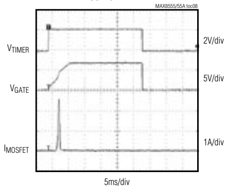
POWER-UP AND DOWN WAVEFORMS USING TIMER
