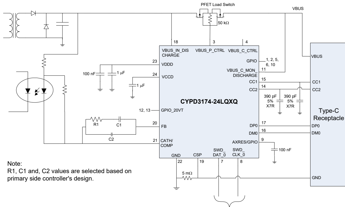
Figure 7. CCG3PA Based Power Adapter Application Diagram with Opto Coupler Feedback Control (24-pin QFN Device)
