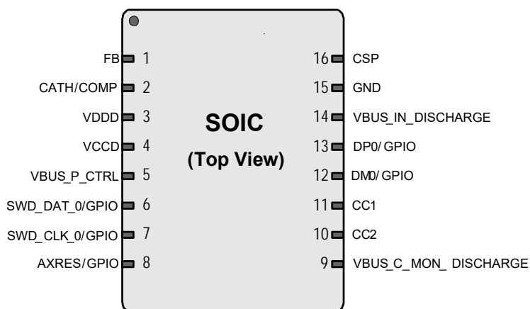
Figure 3. Pinout of 16-SOIC Package (Top View)
