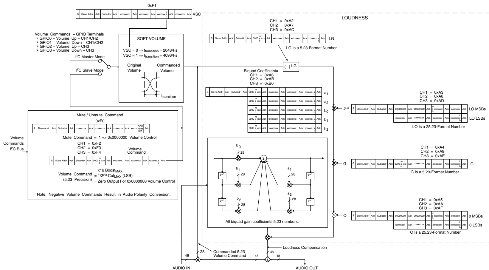
Figure 3–18. Detailed Block Diagram—Soft Volume and Loudness Compensation
