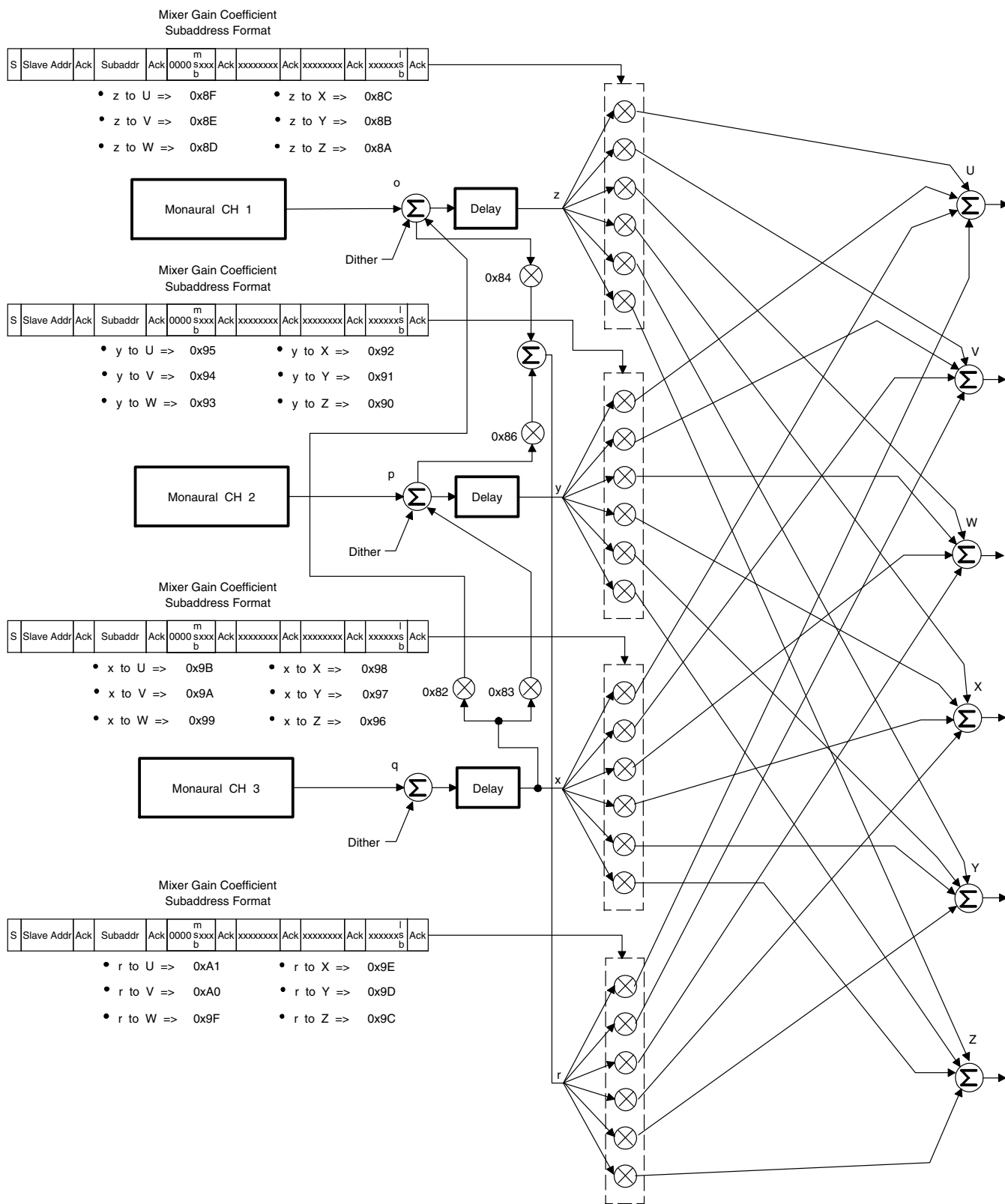
Figure 3–36. Output Crossbar Mixer Topology
