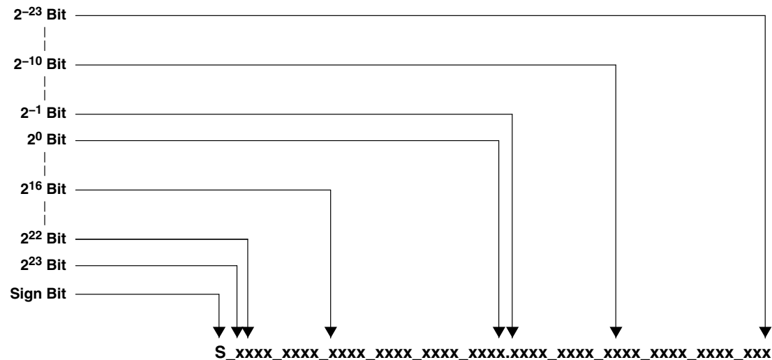
Figure 3–4. 25.23 Format
