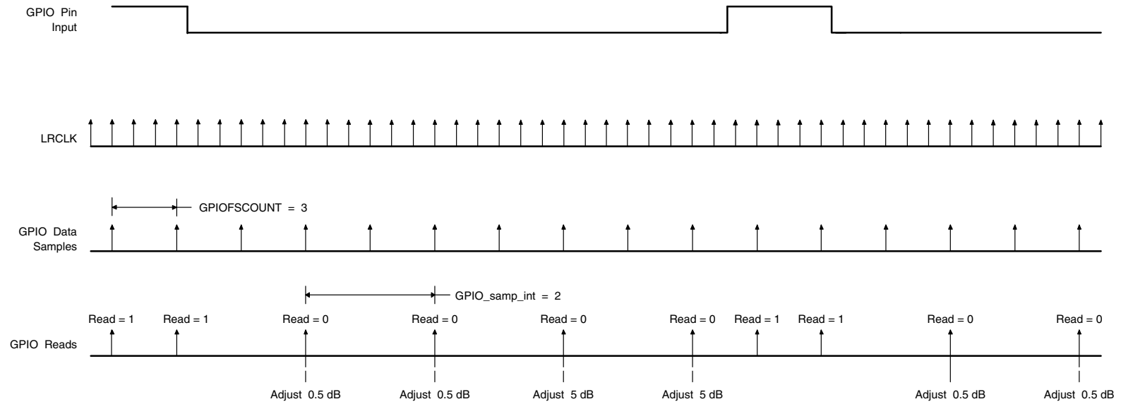
Figure 2-24. Volume Adjustment Timing—Master I 2 C Mode
