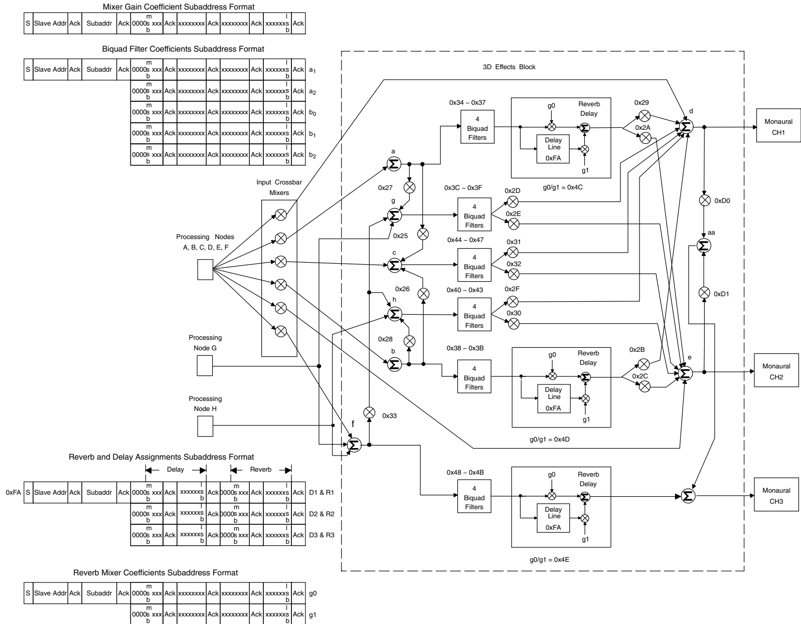
Figure 3–10. TAS3103A 3D Effects Processing Block
