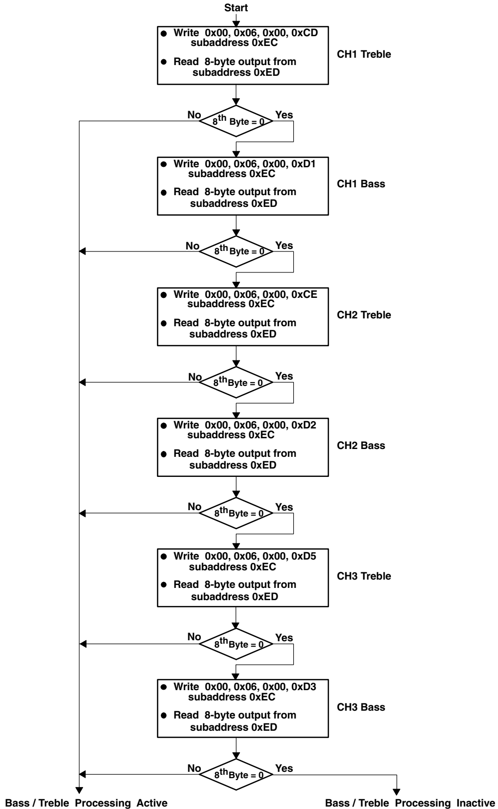
Figure 3–15. I²C Bass/Treble Activity Monitor Procedure
