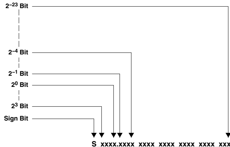
Figure 3–1. 5.23 Format
