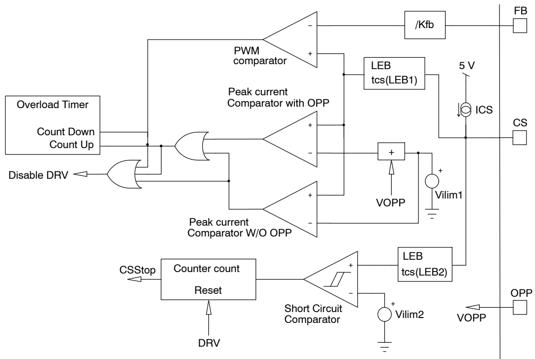
Figure 57. Overload Circuitry
