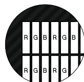
DETAIL A (Dot Size) (NTS)
