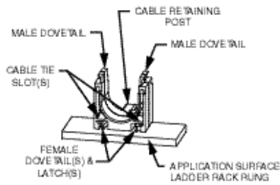
View 2 (CRS1-X and CRS1-125-X)
