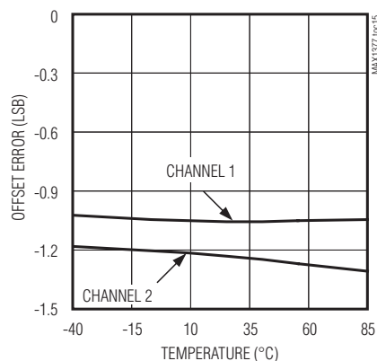
MAX1379 OFFSET ERROR vs. TEMPERATURE
