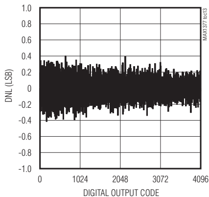
MAX1379 UNIPOLAR DNL vs. DIGITAL OUTPUT CODE
