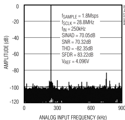
MAX1379 FFT PLOT
