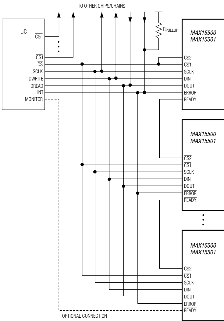
Figure 5. Daisy-Chain Connection (Compatible with Standard SPI)
