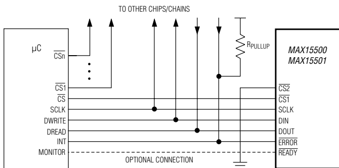
Figure 4. Alternate Single Connection (Compatible with Standard SPI)
