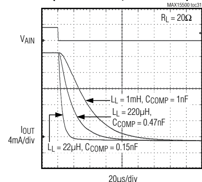
LARGE-SIGNAL SETTLING TIME (CURRENT MODE, FALLING EDGE)
