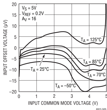
Input Offset Voltage vs Input Common Mode
