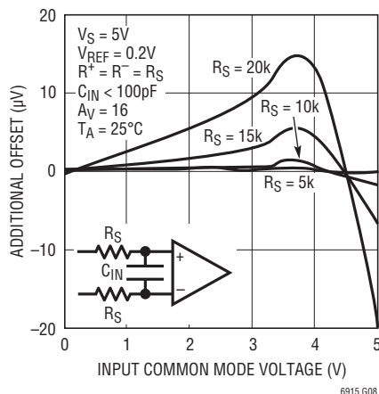
Error Due to Input RS vs Input Common Mode
