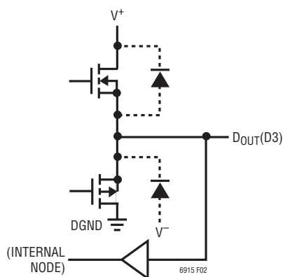
Figure 2. Bidirectional Nature of D_{OUT}/D3 Pin
