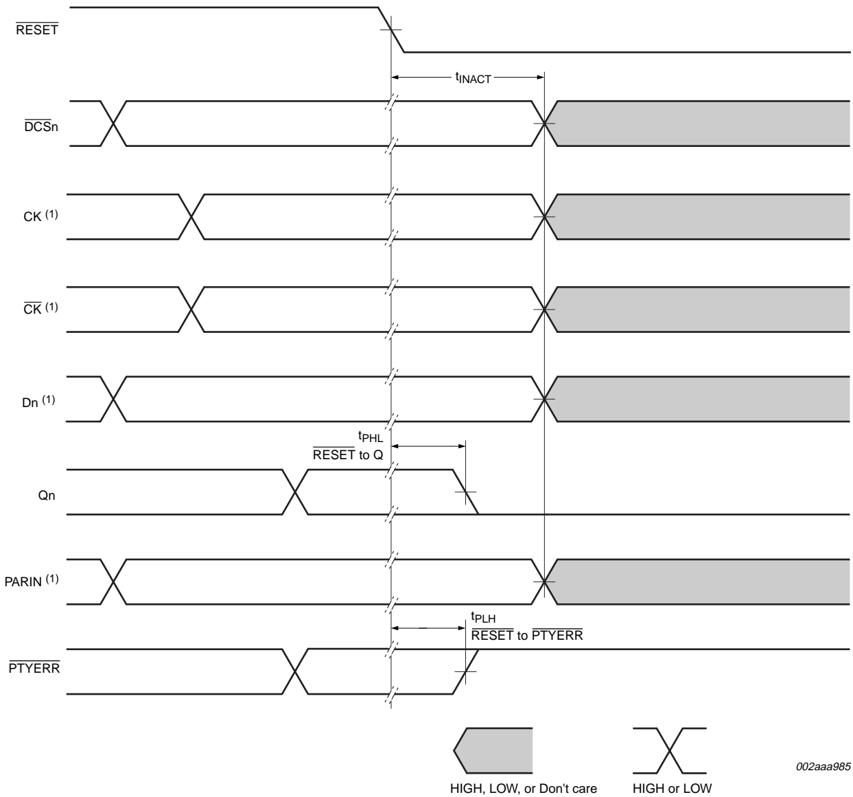
Fig 6. \overline{RESET} switches from HIGH to LOW
