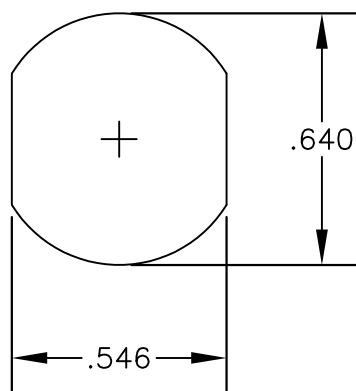
MOUNTING HOLE
