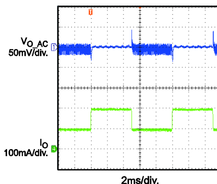
Load Transient I_o = 100mA to 200mA step
