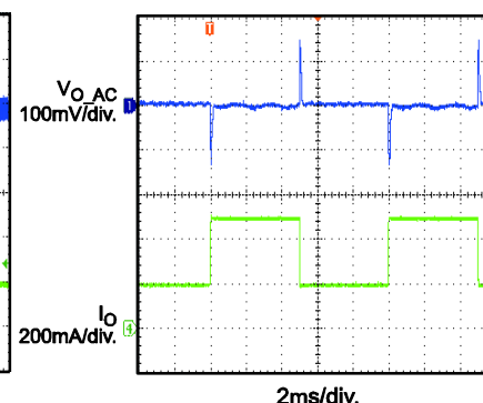
Load Transient I_o = 200mA to 500mA step
