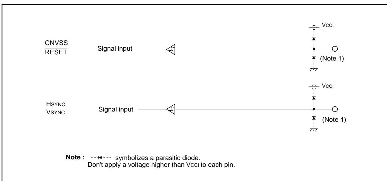
Figure 2.17.5 I/O pins
