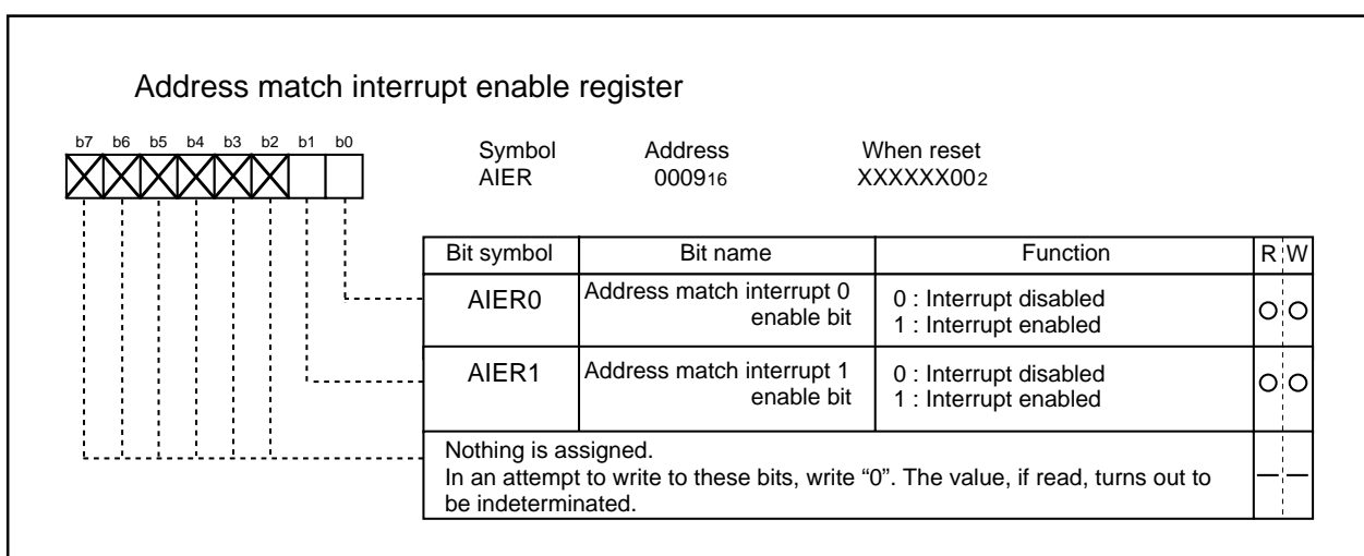
Figure 2.7.12 Address match interrupt enable register
