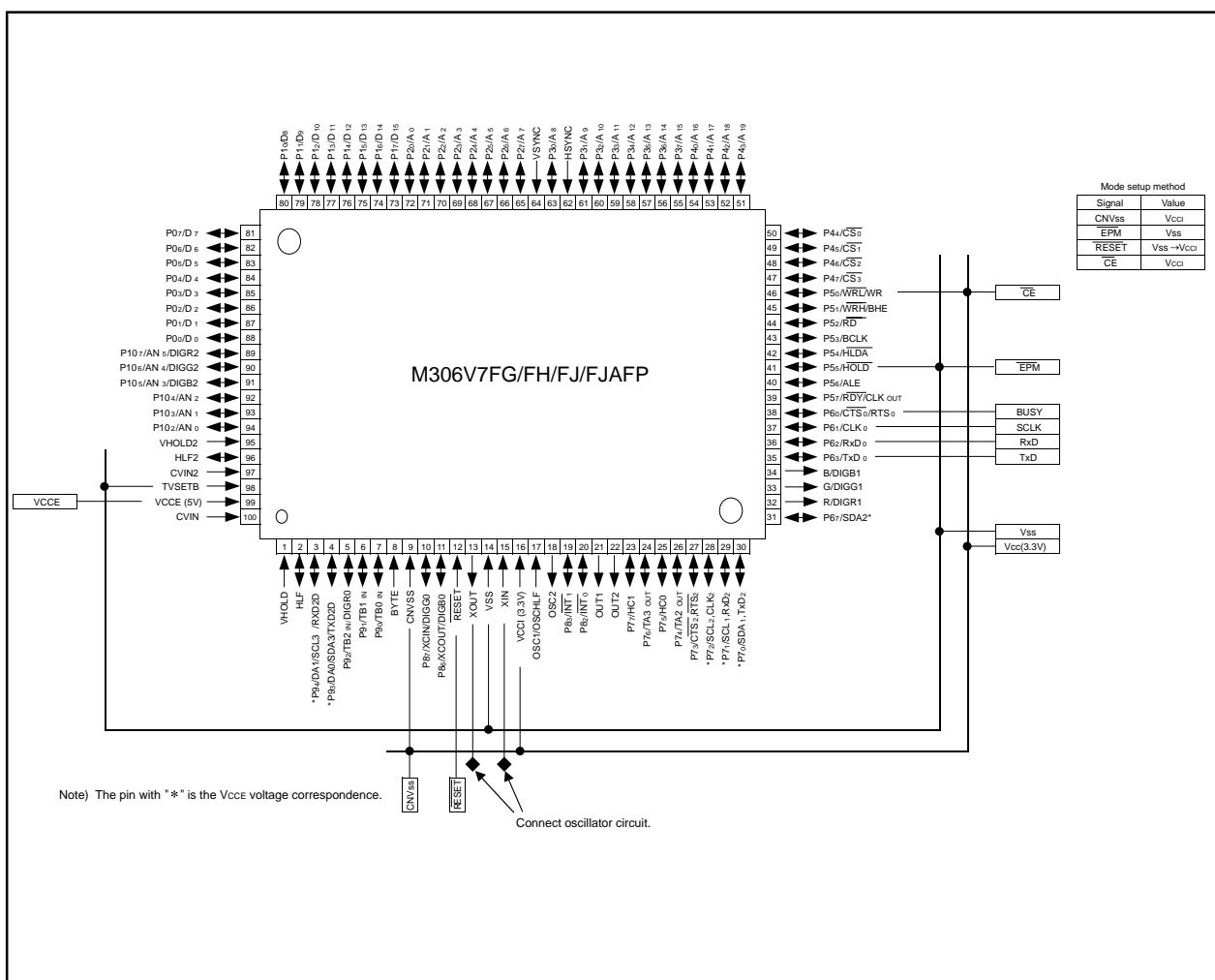
Figure 7.4.1. Pin connections for serial I/O mode (1)
