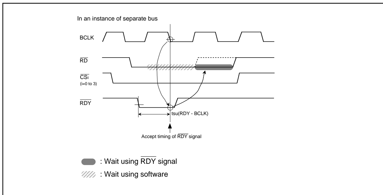
Figure 2.4.5 Example of \overline{\text{RD}} signal extended by \overline{\text{RDY}} signal
