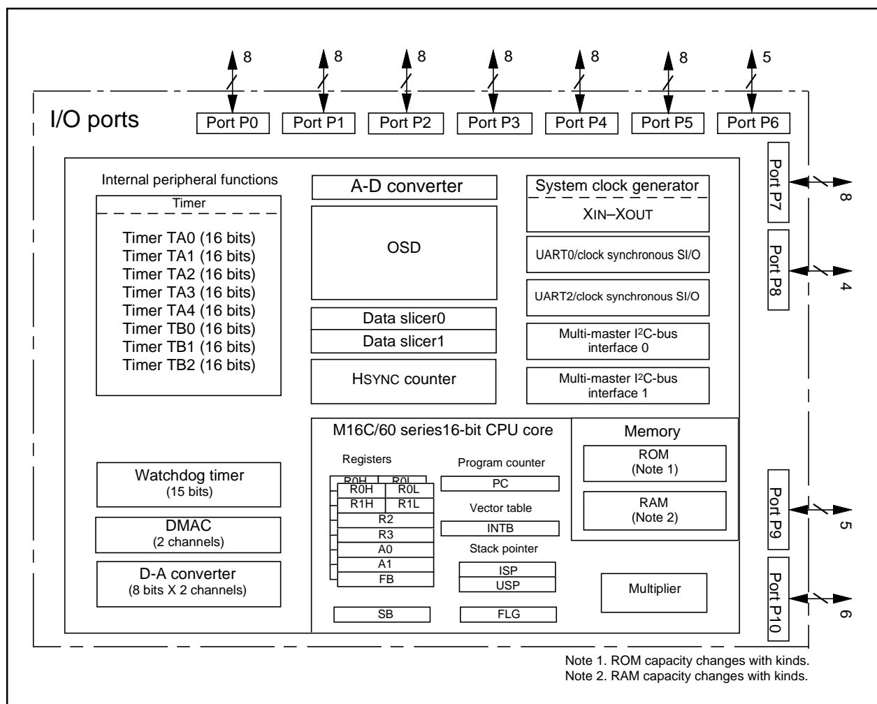
Figure 1.4.1 Block diagram
