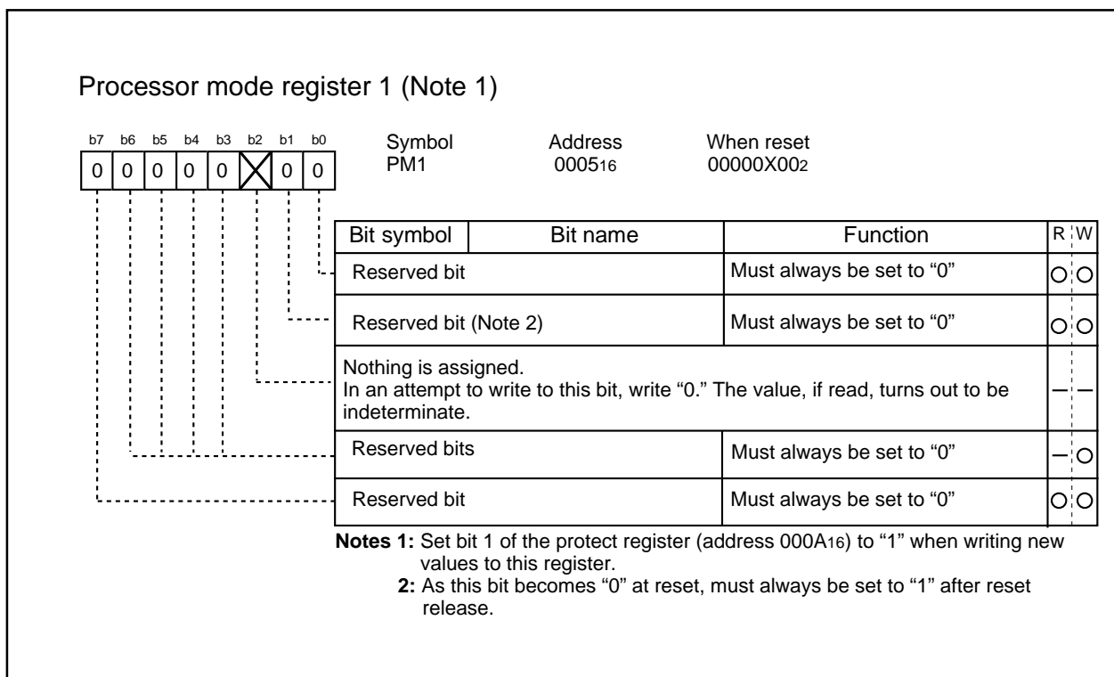
Figure 2.4.2 Processor mode register 1
