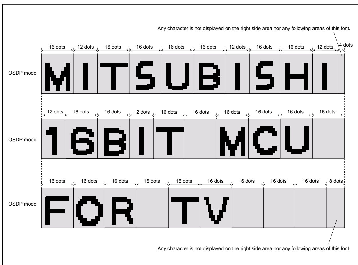
Figure 2.16.38 Display example of OSD mode block
