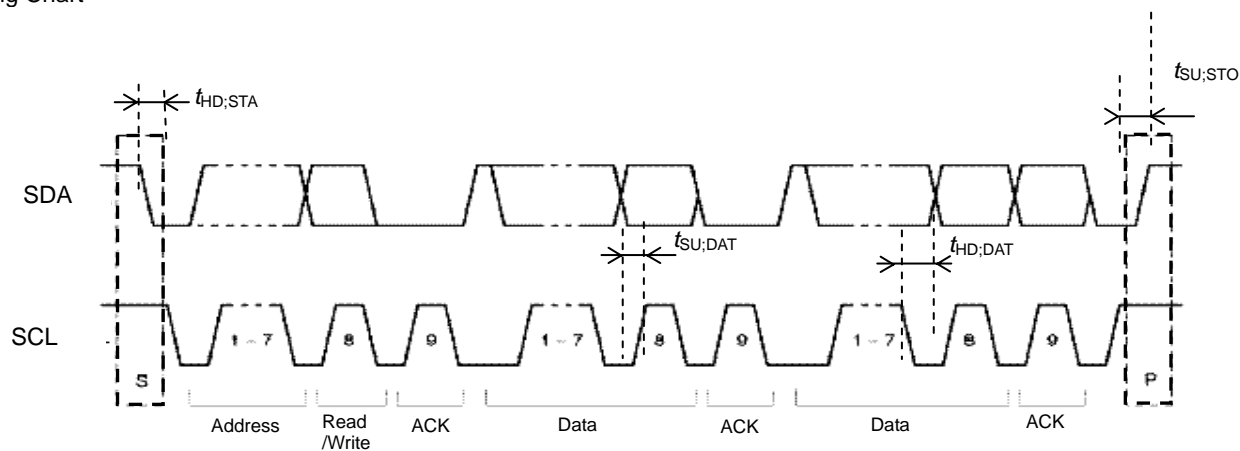
Timing Chart
