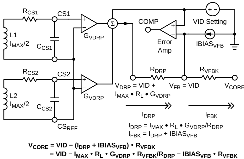
Figure 19. AVP Circuitry at Full-Load
