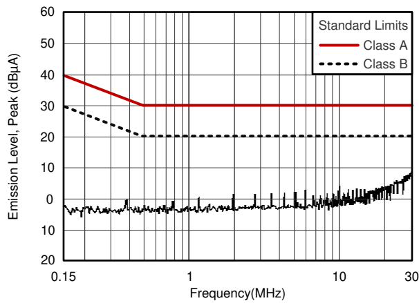
Figure 7-1. Conducted Emissions
