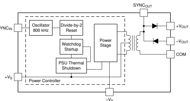
Dual Output Block Diagram
