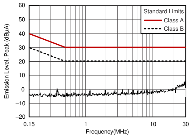
Figure 7-2. Conducted Emissions
