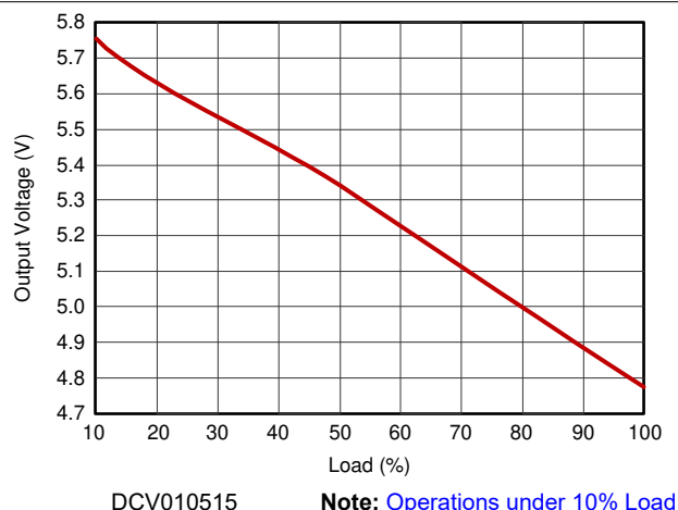
Figure 9-4. Load Regulation
