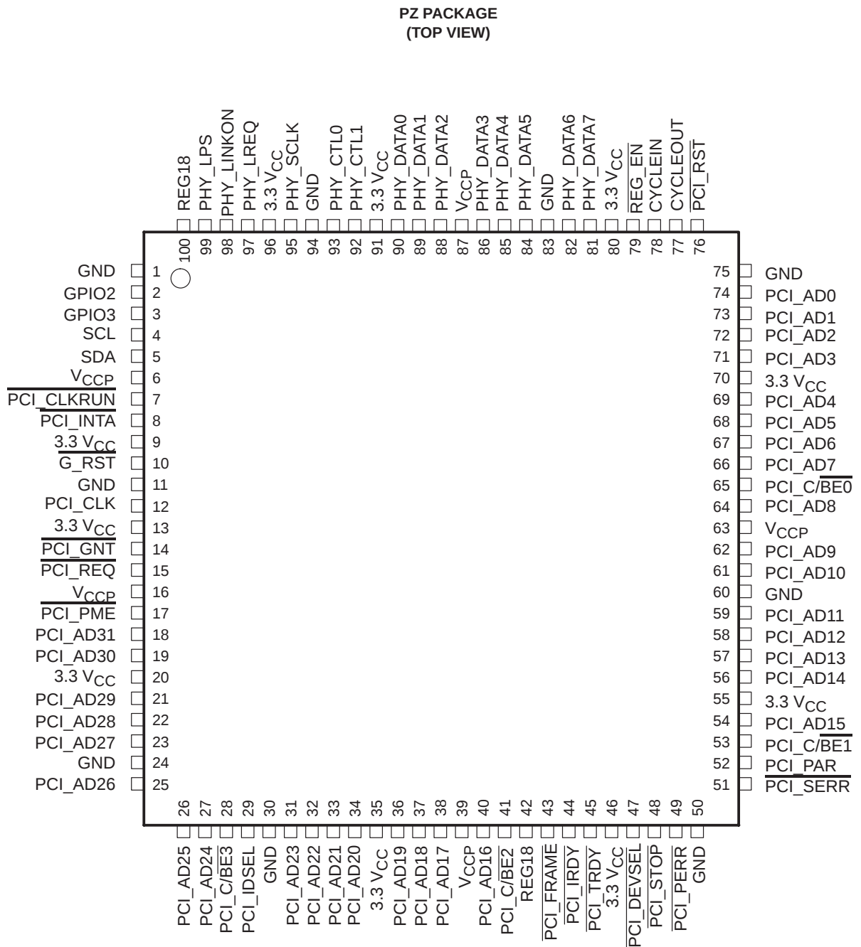
Figure 2–1. Terminal Assignments
